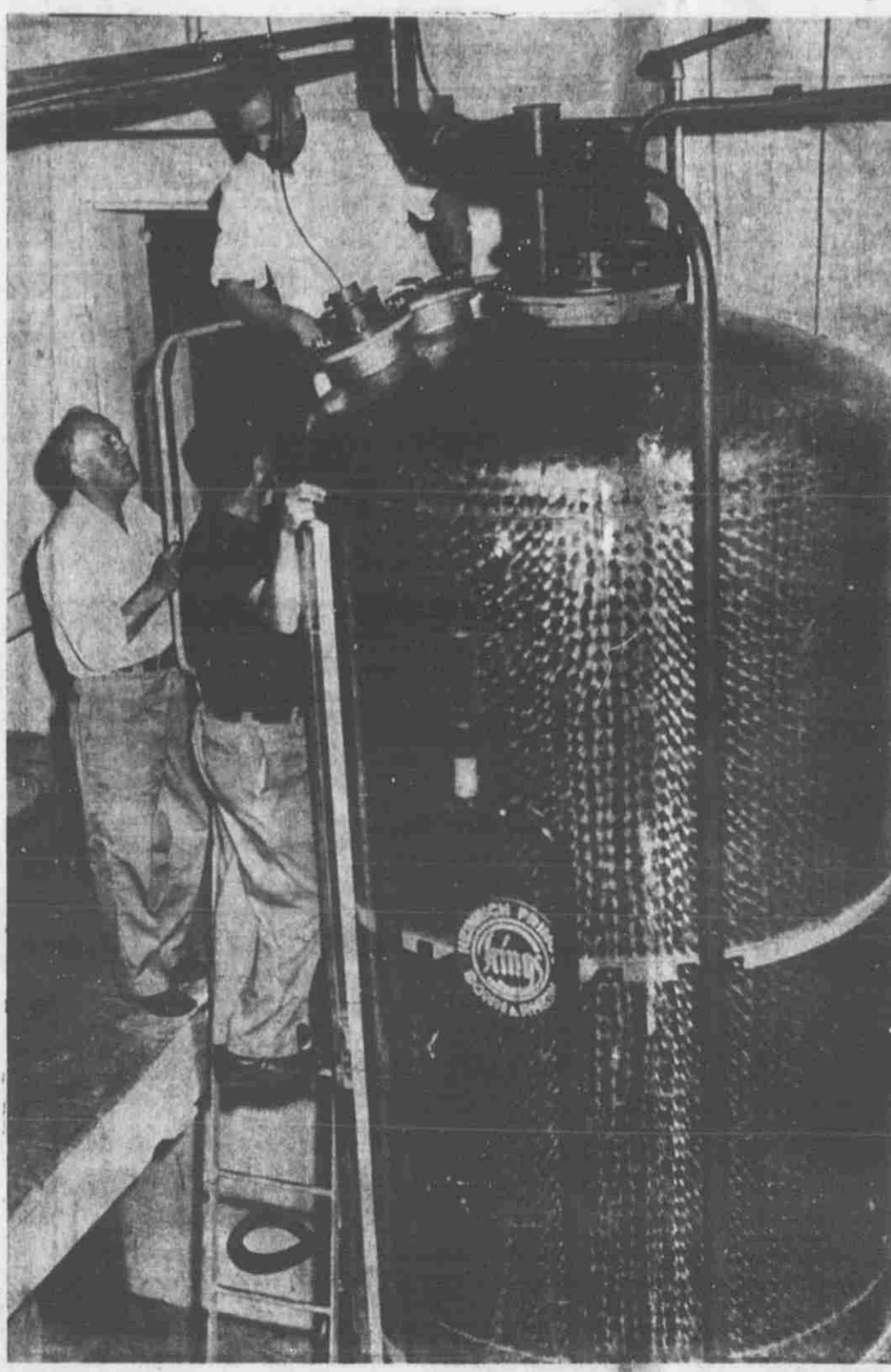
Pictured above, being installed at the Paul Kellogg Vinegar Company plant, is the new ultra-modern generating unit for speeding the process of "making vinegar." It was imported to Lowell from Germany and is the second of this type in America, and first in this part of the country. The men shown in the picture are Kellogg standing on the platform, Ed Kiel on the ladder, and Heinz Ebner, of Germany, at the top.
